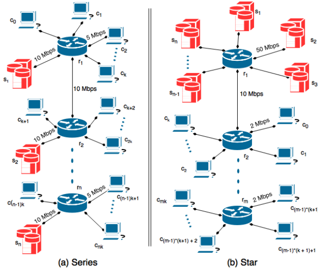
Fig. 2: Simulated topologies.
